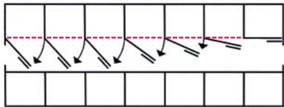
Stall scheme with full swing fronts
