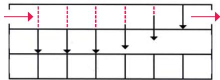
Stable scheme with sliding partitions
